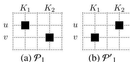
Fig. 6. Persegrams of two equivalent structures.
