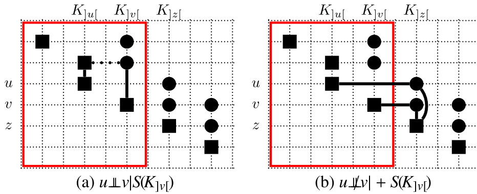
Fig. 9. A contra-example that Lemma 3.9 cannot be generalised.
