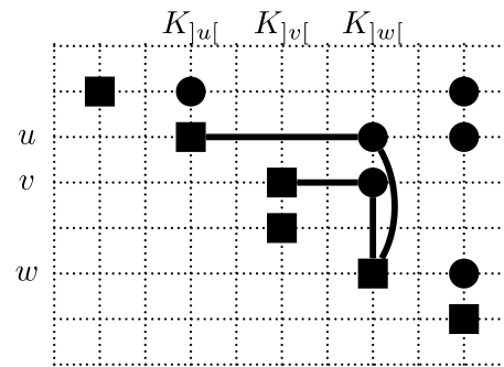
Fig. 10. u \perp\!\!\!\perp v \mid w .
