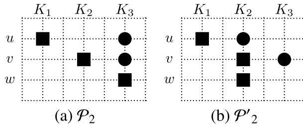
Fig. 7. Persegrams of two non-equivalent structures.
