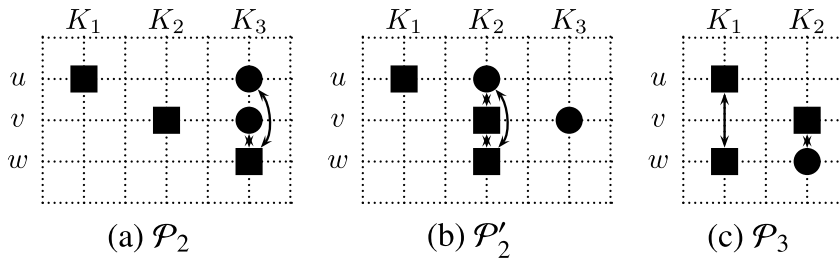
Fig. 8. Connections in different persegrams.
