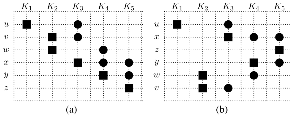
Fig. 1. Different perseggrams belonging to one model structure \mathcal{P} .
